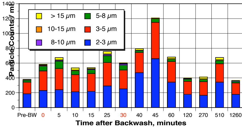
Figure 7. Electronic Particle Count Assessment of Filter Return to Service
