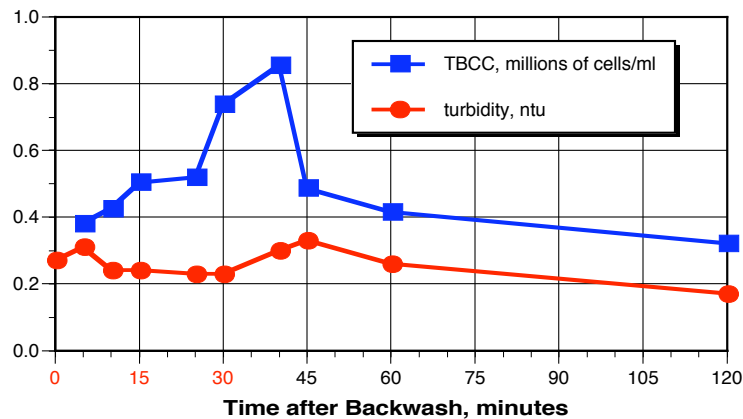
Figure 6. Effect of Ramping during Filter Return to Service
