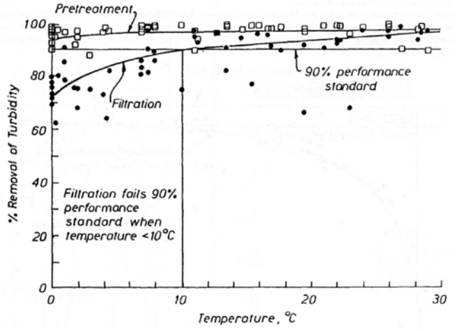
Effect of Missouri River Water Temperature on Percent Removal of Bacteria (Figure 2) and Turbidity (Figure 3) by Pretreatment (Coagulation, Flocculation and Sedimentation) and Rapid Sand Filtration
