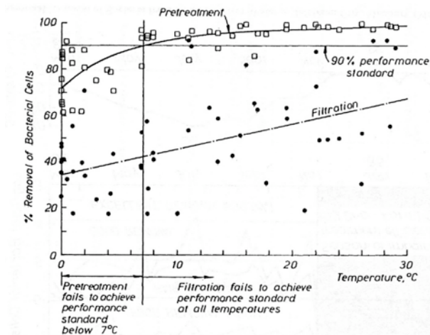
Effect of Missouri River Water Temperature on Percent Removal of Bacteria (Figure 2) and Turbidity (Figure 3) by Pretreatment (Coagulation, Flocculation and Sedimentation) and Rapid Sand Filtration
